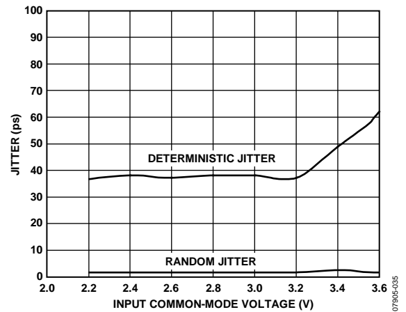
Figure 17. Jitter vs. Input Common-Mode Voltage
