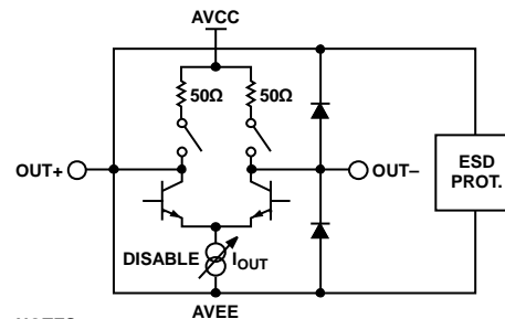
Figure 22. High Speed Output Simplified Schematic
