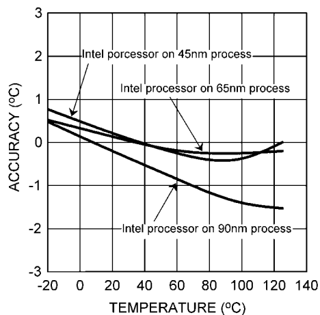
Intel Processor on 45nm, 65nm, or 90 nm Porcess Thermal Diode Performance Comparison
