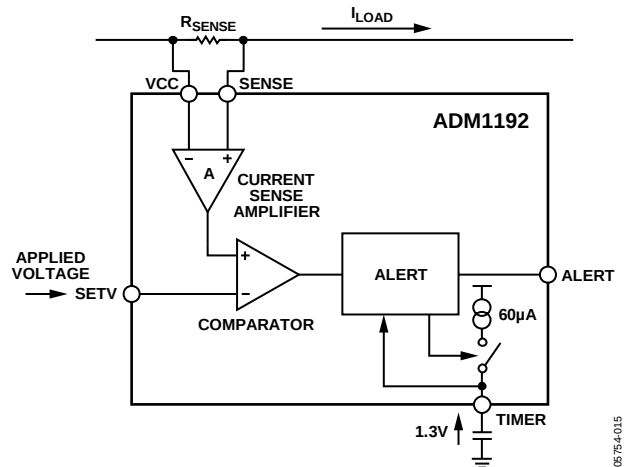
Figure 29. SETV Operation
