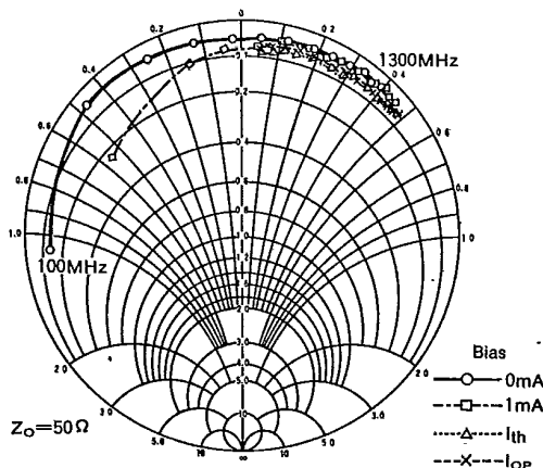
Fig. 12 Impedance characteristics
