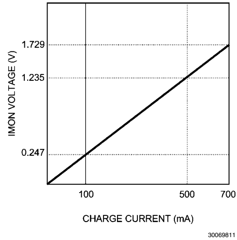
FIGURE 7. IMON Voltage vs. Charge Current
