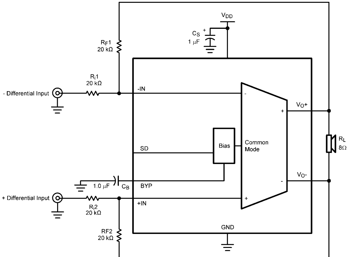
FIGURE 9. Audio Block
