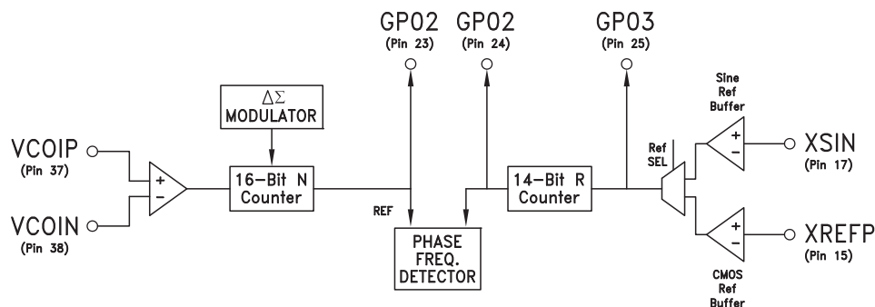
Figure 12. gpo_01 Outputs
