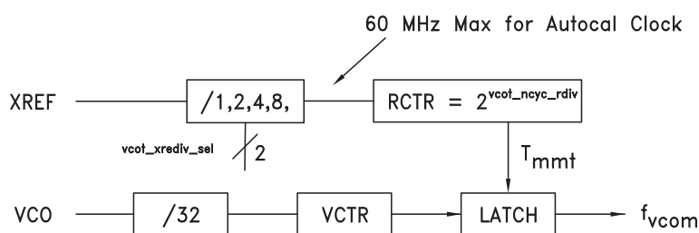
Figure 18. VCO Calibration
