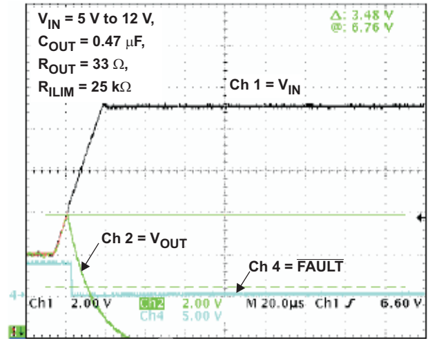
Figure 4. bq24316 OVP Response for Input Step, t_R = 20\ \mu\text{s}
