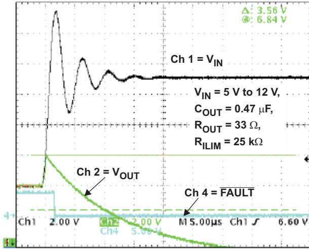
Figure 3. bq24316 OVP Response for Input Step, t_R = 1\ \mu\text{s}
