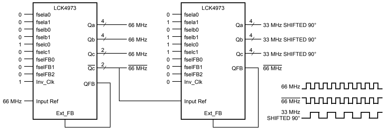
Figure 6. Phase Delay Example Using Two LCK4973s
