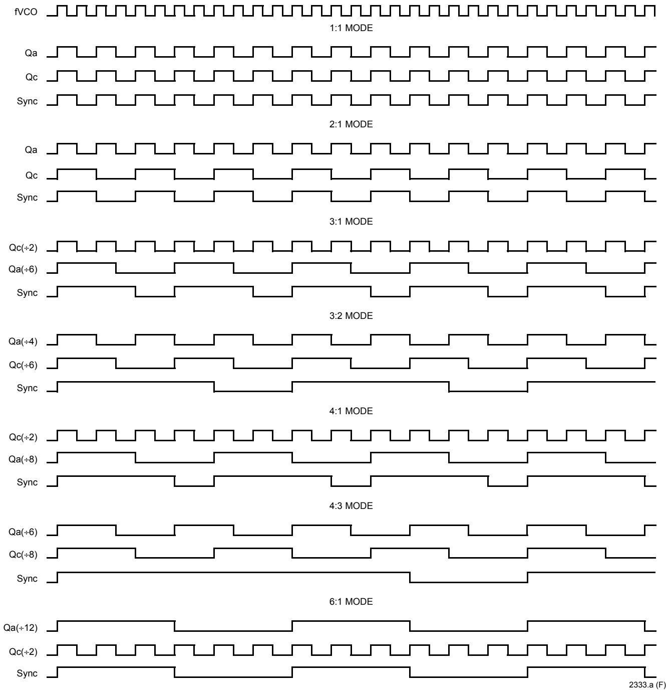
Figure 8. LCK4973 Timing
