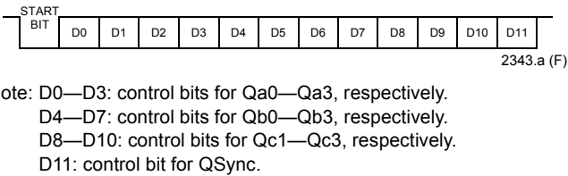
Figure 13. Freeze Data Input Protocol
