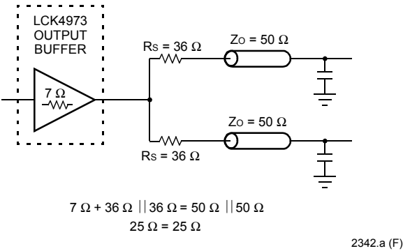
Figure 12. Optimized Dual Transmission Lines
