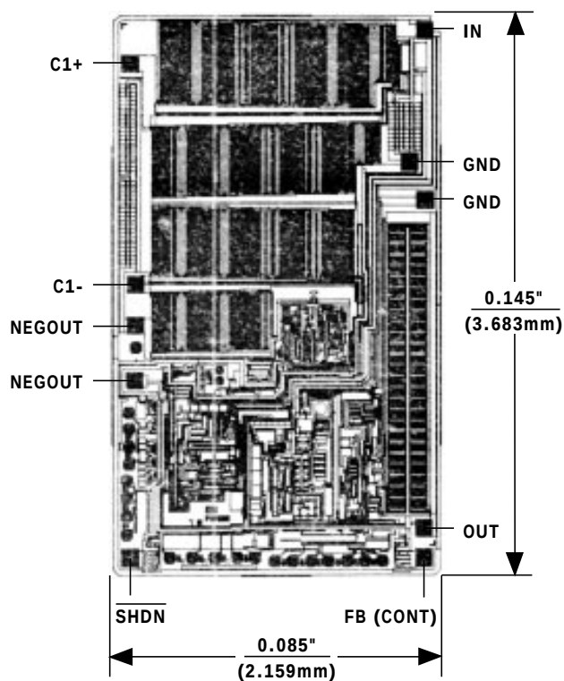
Chip Topography
