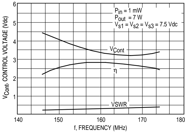
Figure 2. Control Voltage, Efficiency and VSWR versus Frequency
