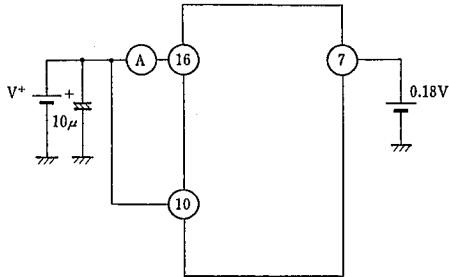
Test Circuit 13
