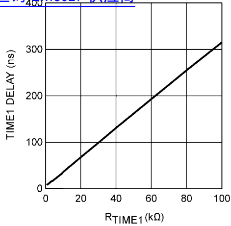
Time1 Delay vs R_{TIME1} (k \Omega )
