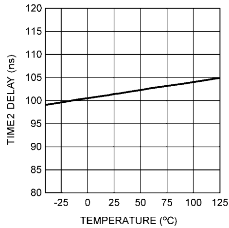
Time2 Delay vs Temperature R_{TIME2} = 28.7 k \Omega
