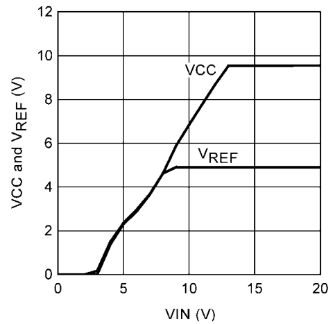
VCC and V REF vs. V IN
