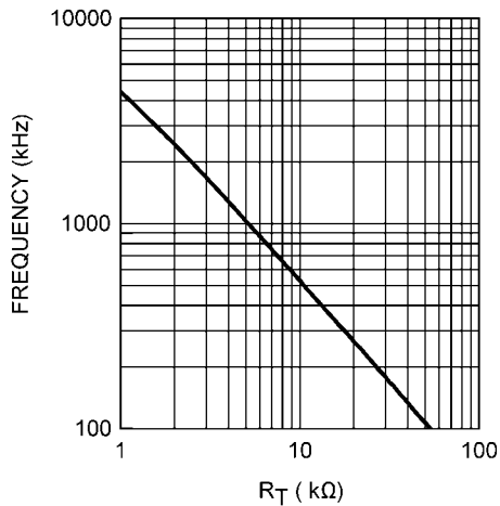
Oscillator Frequency vs R T Resistor
