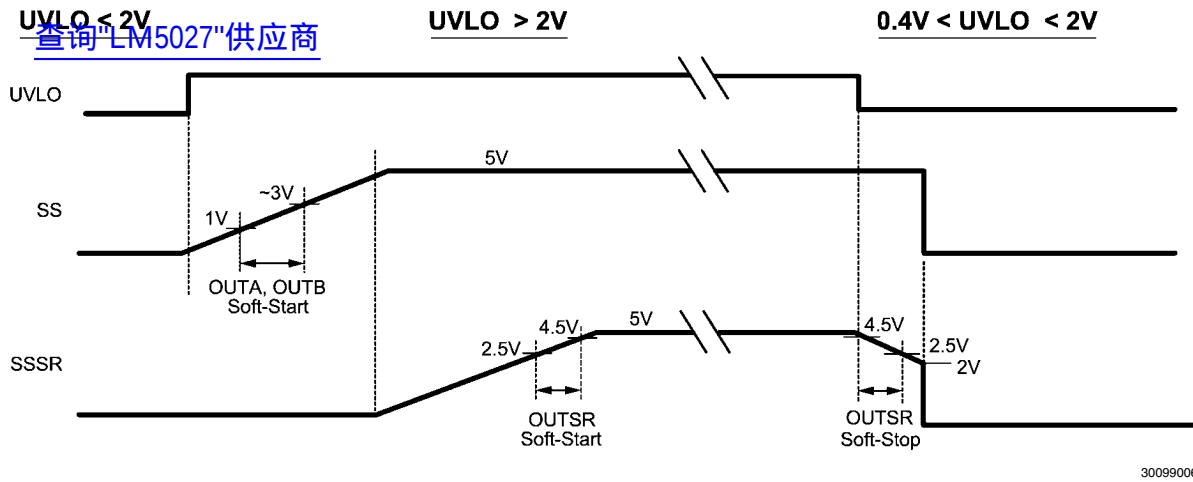
FIGURE 4. Soft-Start/Soft-Stop Timing
