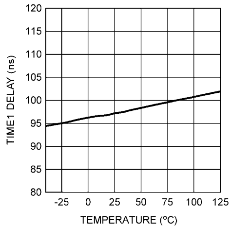
Time1 Delay vs Temperature R_{TIME1} = 33.2 k \Omega
