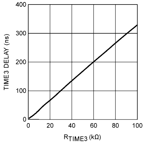
Time3 Delay vs R_{TIME3} (k \Omega )
