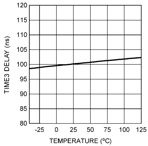
Time3 Delay vs Temperature R_{TIME3} = 29.4 k \Omega
