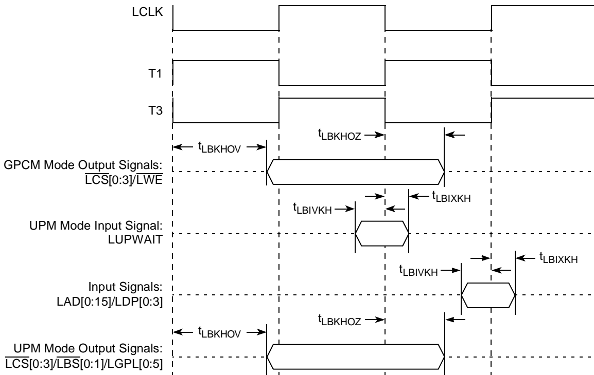
Figure 16. Local Bus Signals, GPCM/UPM Signals for LCCR[CLKDIV] = 2
