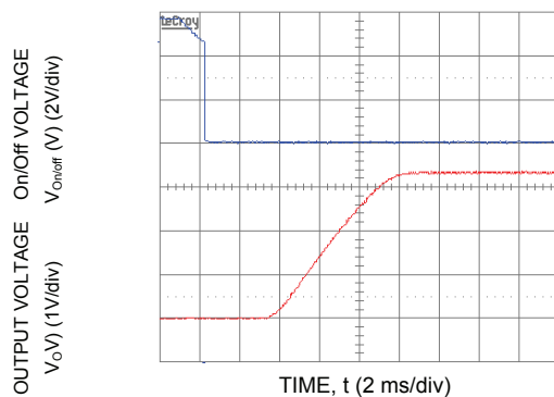
Figure 15. Typical Start-Up Using Remote On/Off with Low-ESR external capacitors ( V_{in} = 5.5\text{ Vdc} , V_o = 3.3\text{ Vdc} , I_o = 10.0\text{ A} , C_o = 1050\text{ }\mu\text{F} ).
