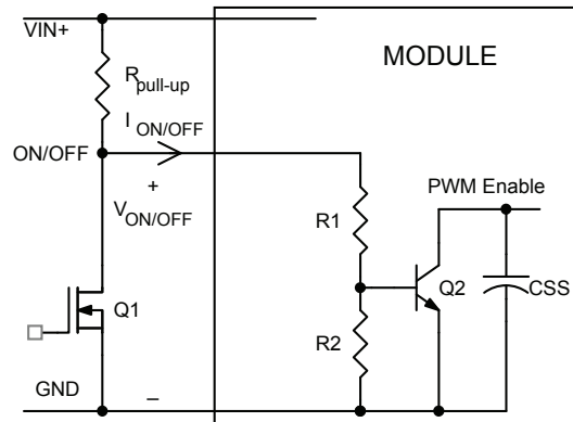
Figure 30. Circuit configuration for using negative logic On/Off.
