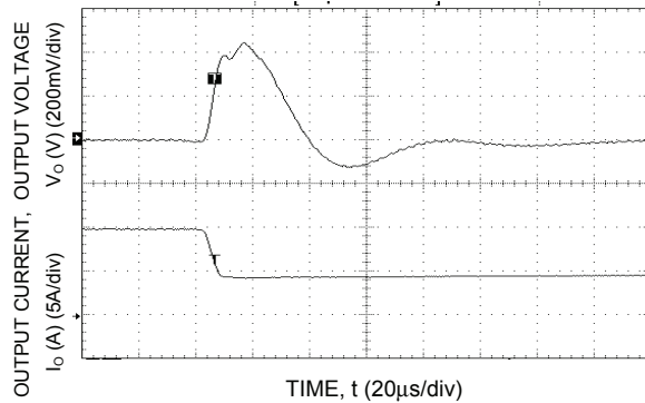
Figure 13. Transient Response to Dynamic Load Change from 100% of 50% full load ( V_o = 3.3\text{ Vdc} , C_{ext} = 2 \times 150\text{ }\mu\text{F} Polymer Capacitors).
