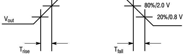
Figure 14. Waveforms: Rise and Fall Times
