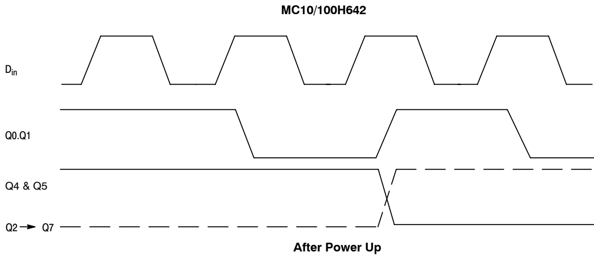
Figure 11. Q2 → Q7 will Synchronize with Pos Edges of D_{in} & Q0 \rightarrow Q1 Outputs
