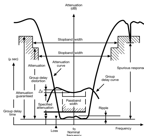
Figure 3) MCF Characteristics Curve
