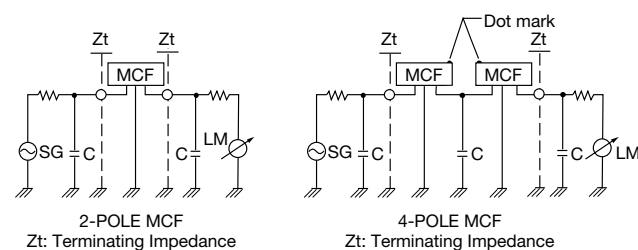
Figure 5) MCF Test Circuits
