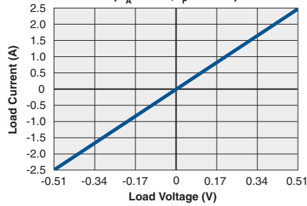
CPC1927 Typical Load Current vs. Load Voltage ( T_A = 25°C, I_F = 10mA )
