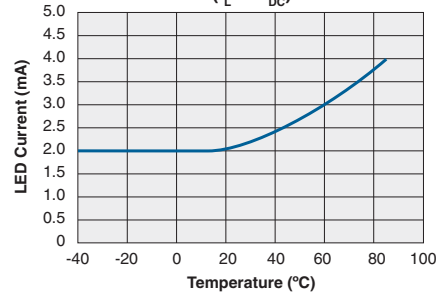
CPC1927 Typical I_F for Switch Operation vs. Temperature ( I_L = 1A_{DC} )
