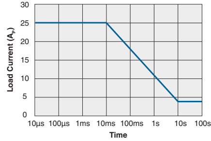
CPC1927 Energy Rating Curve (Free Air, No Heat Sink)
