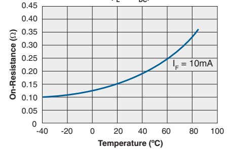
CPC1927 Typical On-Resistance vs. Temperature ( I_L = 1A_{DC} )
