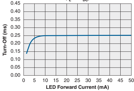
CPC1927 Typical Turn-Off vs. LED Forward Current ( I_L = 1A_{DC} )
