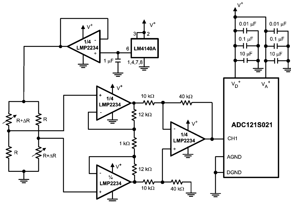
Strain Gauge Bridge Amplifier
