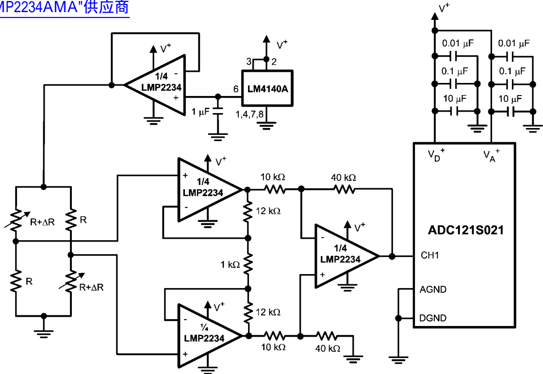
FIGURE 5. Strain Gauge Bridge Amplifier
