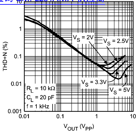
THD+N vs. Amplitude 查询"LMP2234AMA"供应商
