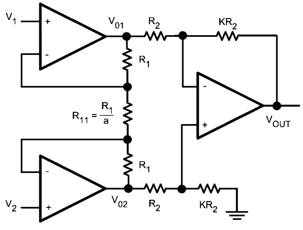
FIGURE 3. Instrumentation Amplifier
