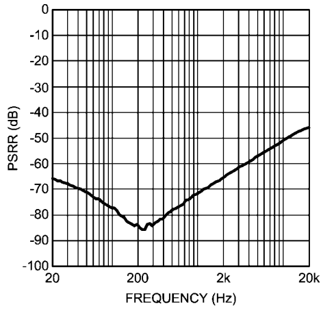
PSRR vs Frequency V_{DD} = 5V , R_L = 32\Omega , C_{BYP} = 2.2\mu F V_{RIPPLE} = 200mV_{p-p} , MODE 8, OCL
