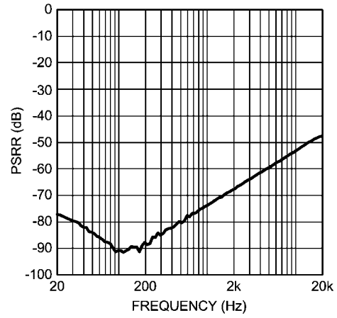
PSRR vs Frequency V_{DD} = 5V , R_L = 32\Omega , C_{BYP} = 2.2\mu F V_{RIPPLE} = 200mV_{p-p} , MODE 8, SE
