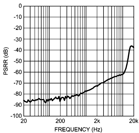
PSRR vs Frequency V_{DD} = 3.3V , R_L = 8\Omega , C_{BYP} = 2.2\mu F V_{RIPPLE} = 200mV_{P-P} , MODE 1
