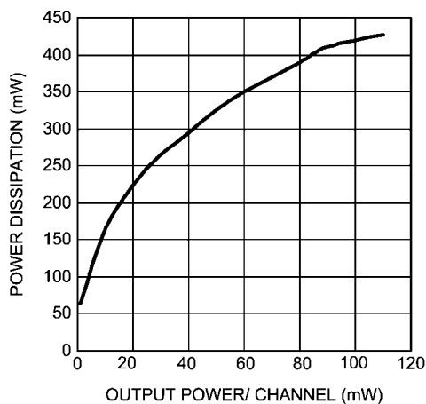
Power Dissipation vs Output Power V_{DD} = 5V , R_L = 32\Omega f = 1kHz , Mode 8, OCL
