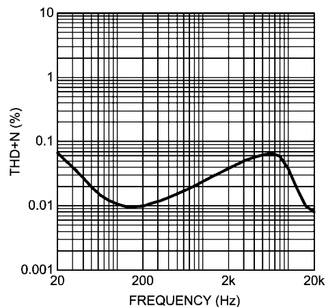
THD+N vs Frequency V_{DD} = 3.3V , R_L = 32\Omega , P_O = 12mW f = 22kHz , Mode 8, OCL
