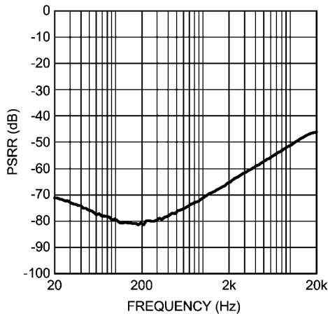
PSRR vs Frequency V_{DD} = 5V , R_L = 64\Omega , C_{BYP} = 4.7\mu F V_{RIPPLE} = 200mV_{p-p} , MODE 4, BTL
