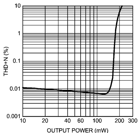
THD+N vs Output Power V_{DD} = 5V , R_L = 64\Omega f = 1kHz , Mode 4, BTL
