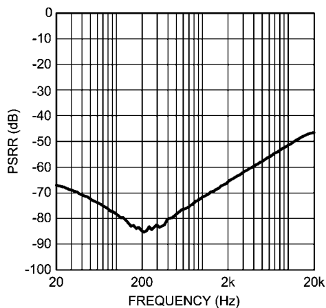
PSRR vs Frequency V_{DD} = 3.3V , R_L = 32\Omega , C_{BYP} = 2.2\mu F V_{RIPPLE} = 200mV_{P-P} , MODE 8, OCL
