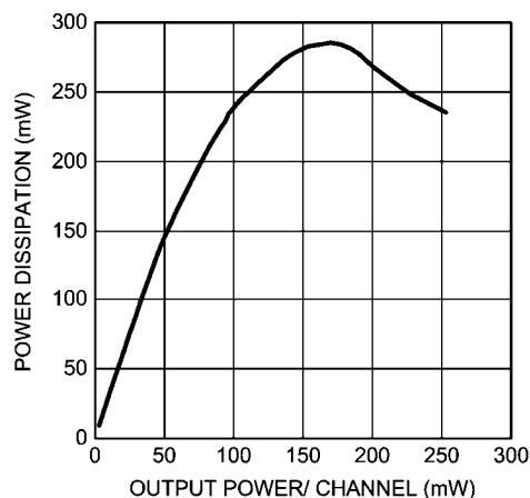
Power Dissipation vs Output Power V_{DD} = 3.3V , R_L = 8\Omega f = 1kHz , Mode 1, Speaker
