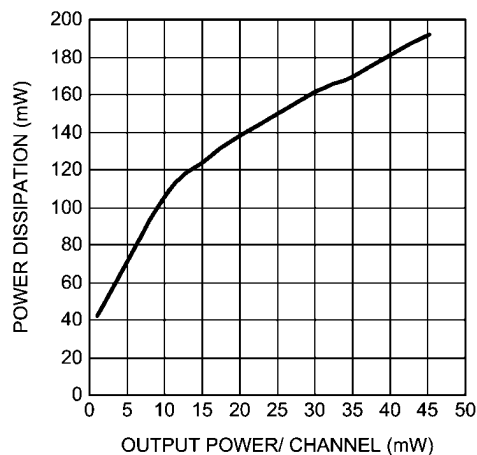
Power Dissipation vs Output Power V_{DD} = 3.3V , R_L = 32\Omega f = 1kHz , Mode 8, OCL
