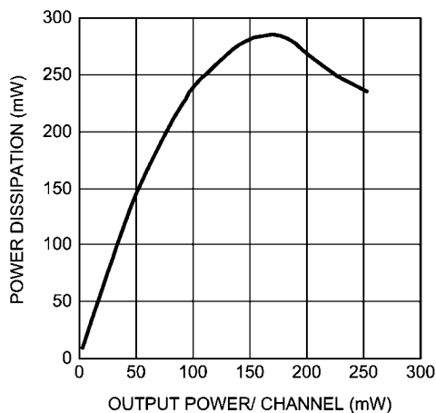
Power Dissipation vs Output Power V_{DD} = 5V , R_L = 8\Omega f = 1kHz , Mode 1, Speaker
