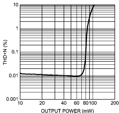
THD+N vs Output Power V_{DD} = 5V , R_L = 32\Omega f = 1kHz , Mode 8, SE
