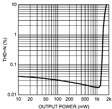
THD+N vs Output Power V_{DD} = 5V , R_L = 8\Omega f = 1kHz , Mode 1, Speaker
