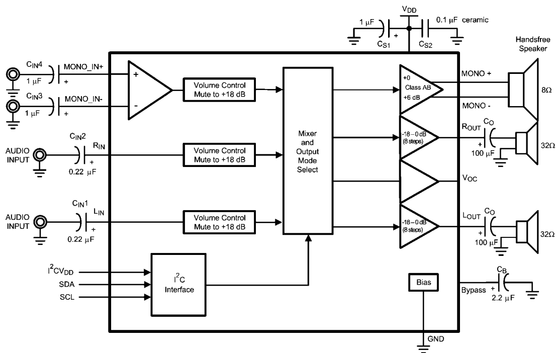
FIGURE 2. Single-Ended Configuration
