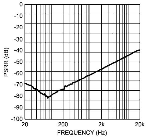
PSRR vs Frequency V_{DD} = 5V , R_L = 32\Omega , C_{BYP} = 4.7\mu F V_{RIPPLE} = 200mV_{p-p} , MODE 8, SE
