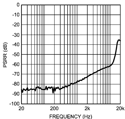
PSRR vs Frequency V_{DD} = 3.3V , R_L = 8\Omega , C_{BYP} = 4.7\mu F V_{RIPPLE} = 200mV_{P-P} , MODE 1
