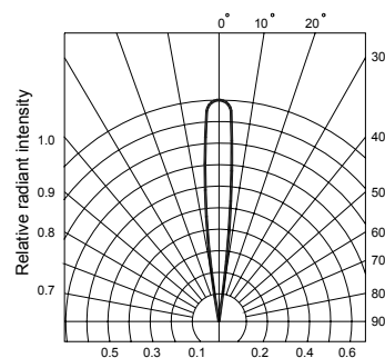
Fig.6 Radiation diagram
