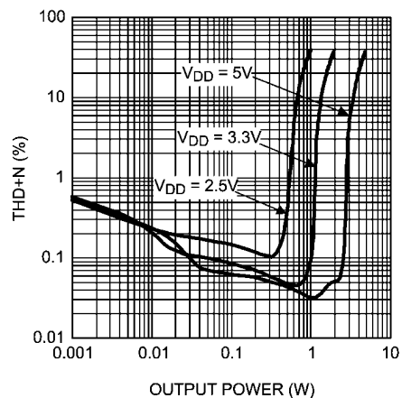
THD+N vs Output Power A_V = 12\text{dB} , f = 1\text{kHz} , R_L = 3\Omega
