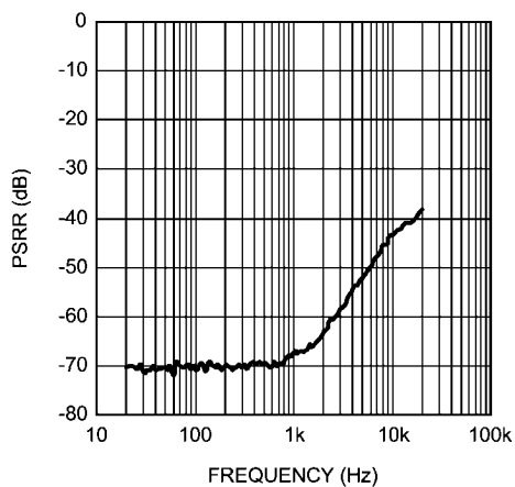
PSRR vs Frequency V_{DD} = 5\text{ V}, V_{\text{RIPPLE}} = 200\text{ mV}_{\text{P-P}}, R_L = 8\Omega
