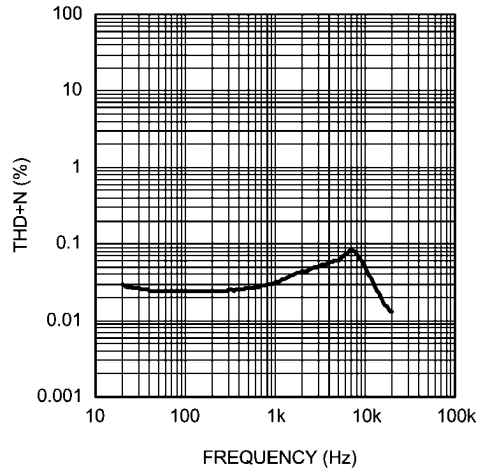
THD+N vs Frequency V_{DD} = 5V , P_O = 1W , R_L = 8\Omega
