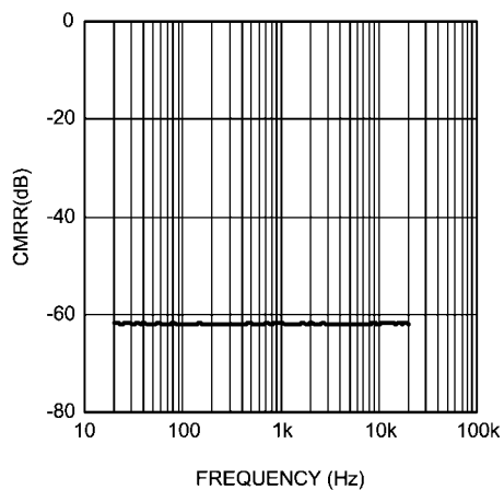
CMRR vs Frequency V_{DD} = 5\text{ V}, V_{\text{RIPPLE}} = 1\text{ V}_{\text{P-P}}, R_L = 8\Omega
