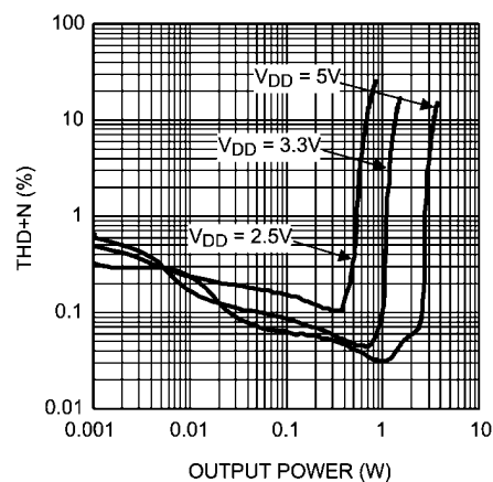
THD+N vs Output Power A_V = 0\text{dB} , f = 1\text{kHz} , R_L = 3\Omega
