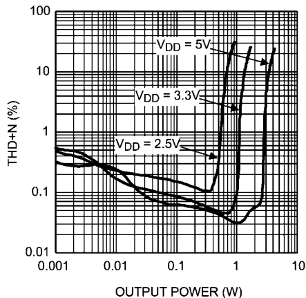
THD+N vs Output Power A_V = 30\text{dB} , f = 1\text{kHz} , R_L = 3\Omega
