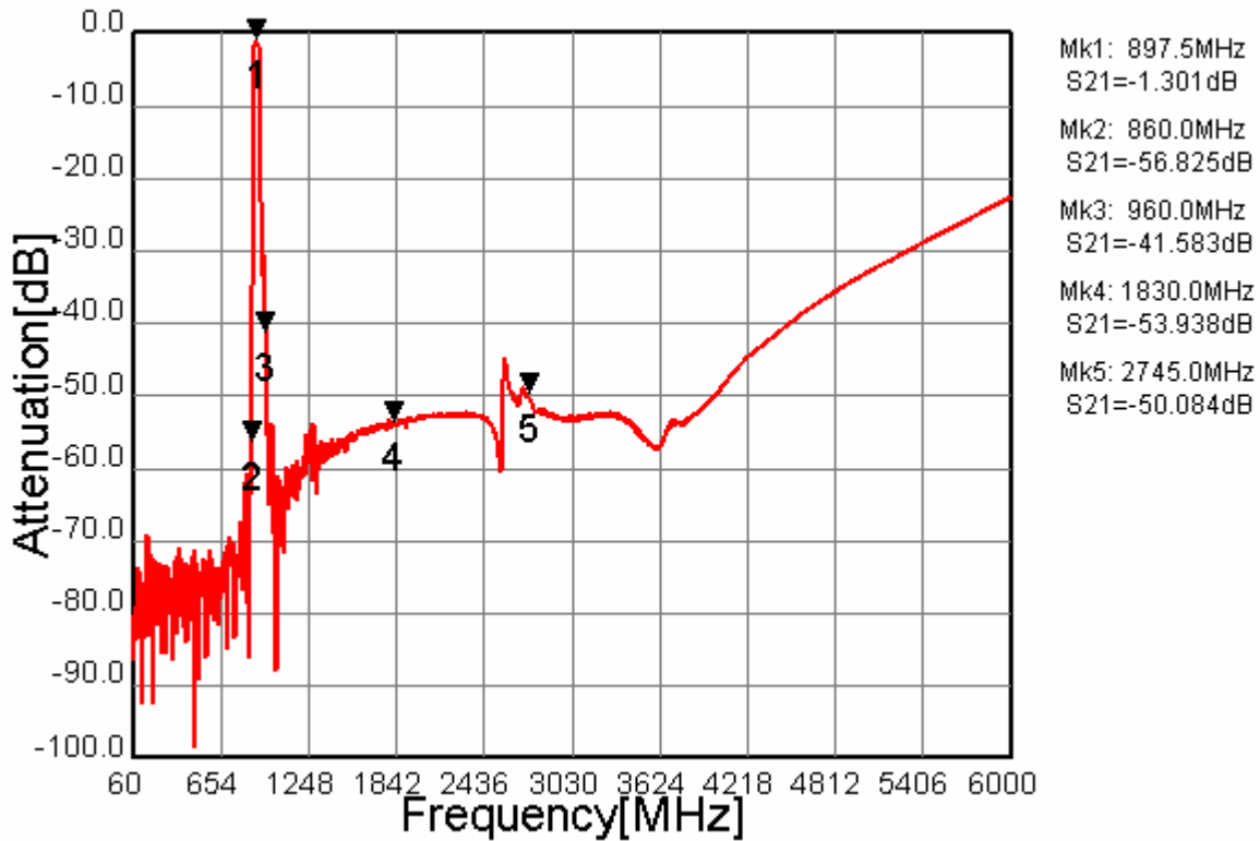
Fig.4 Wide-band Characteristics
