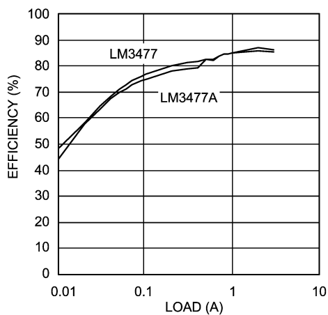
Efficiency vs Load Current ( V_{IN} = 12V , V_{OUT} = 3.3V )
