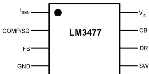
8 Lead Mini SO8 Package (MSOP-8 Package)
