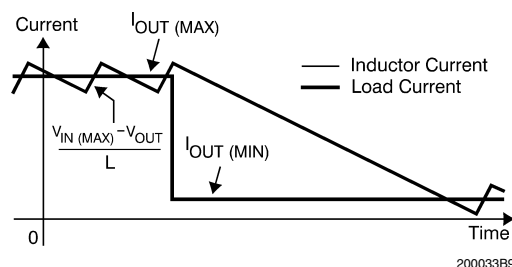
FIGURE 9. A Loading Transient
