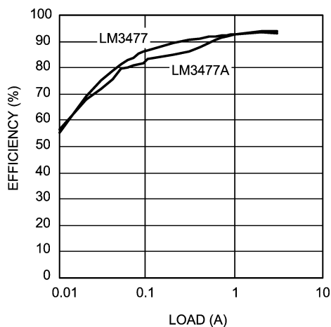
Efficiency vs Load Current ( V_{IN} = 24V , V_{OUT} = 12V )
