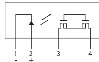
CPC1981Y Pinout
