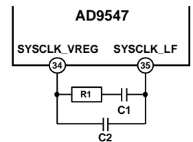
Figure 44. External Loop Filter Schematic
