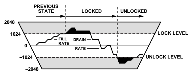
Figure 39. Phase Lock Detector Diagram
