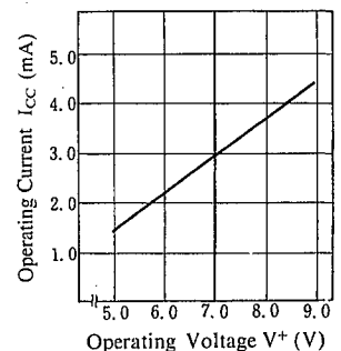
Graph 23 Operating Current vs. Operating Voltage
