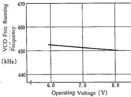
Graph 15 VCO Free Running Frequency vs. Operating Voltage
