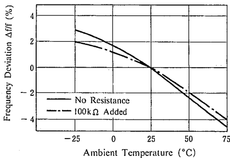
Graph 17 VCO Frequency Deviation vs. Ambient Temperature
