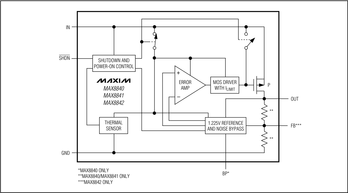
Functional Diagram
