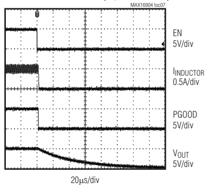
SHUTDOWN WAVEFORM ( I_{LOAD} = 600mA )
