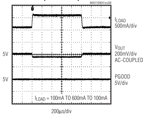
LOAD TRANSIENT RESPONSE (FIXED MODE)
