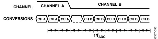
Figure 61. Fast Settling, Sinc 3 Filter
