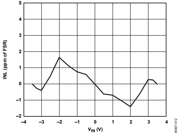
Figure 12. INL (Gain = 1)
