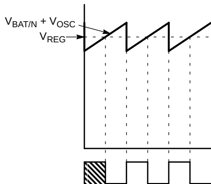
Figure 4. 50% Duty Cycle, Steady State
