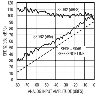
SFDR2 vs. ANALOG INPUT AMPLITUDE ( f_{CLK} = 100MHz , f_{IN} = 70MHz )
