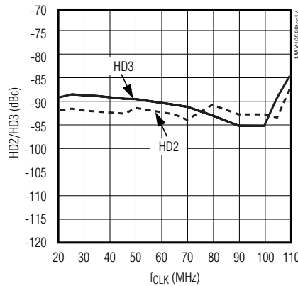
HD2/HD3 vs. SAMPLING FREQUENCY ( f_{IN} = 10MHz , A_{IN} = -2dBFS )
