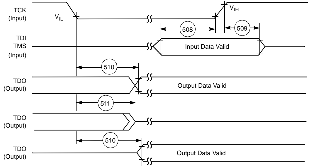
Figure 2-48. Test Access Port Timing Diagram
