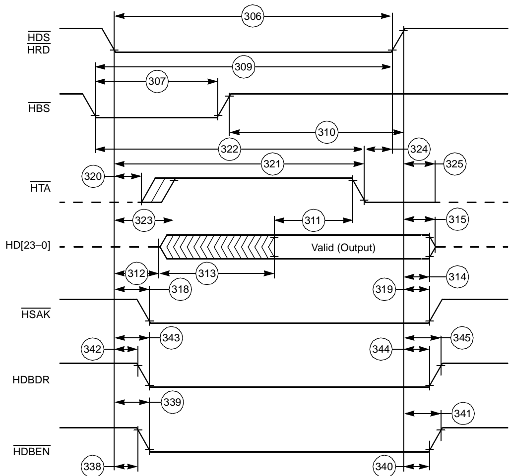
Figure 2-32. Read Timing
