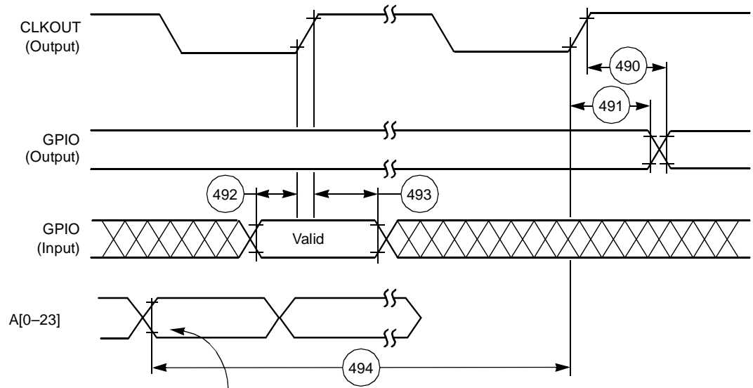
Figure 2-45. GPIO Timing
