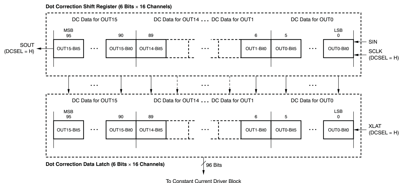
Figure 29. Dot Correction Shift Register and Latch Configuration
