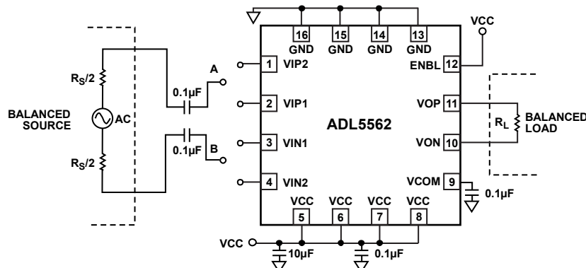
Figure 31. Basic Connections
