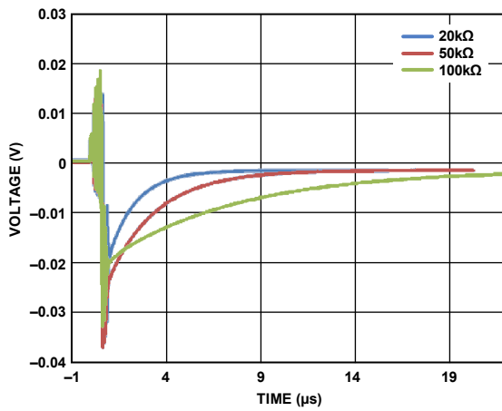
Figure 32. Maximum Glitch Energy
