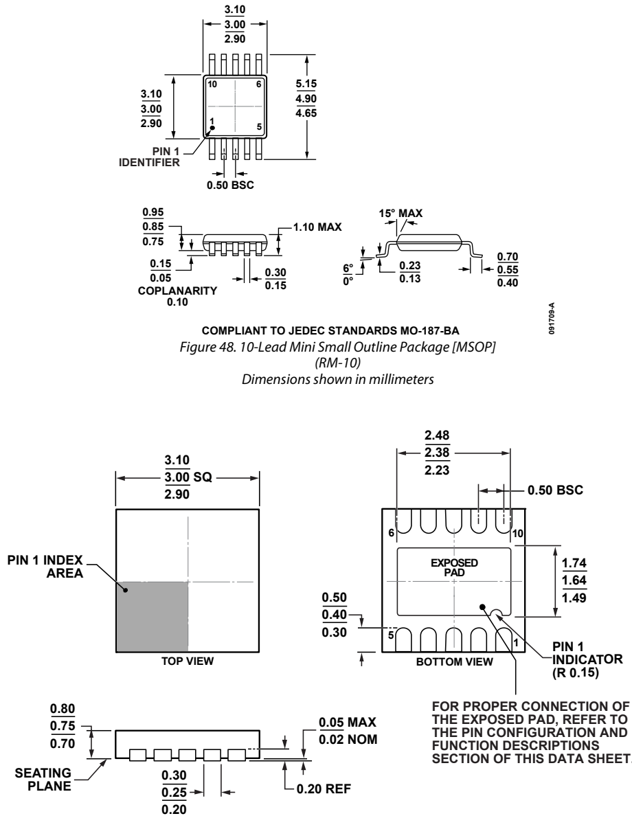
Figure 49. 10-Lead Frame Chip Scale Package [LFCSP_WD] 3 mm × 3 mm Body, Very Thin, Dual Lead (CP-10-9) Dimensions shown in millimeters
