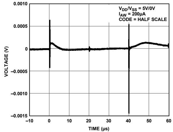
Figure 35. Digital Feedthrough
