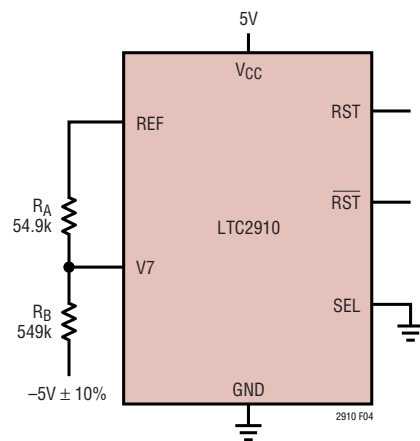
Figure 4. Negative Supply Monitor
