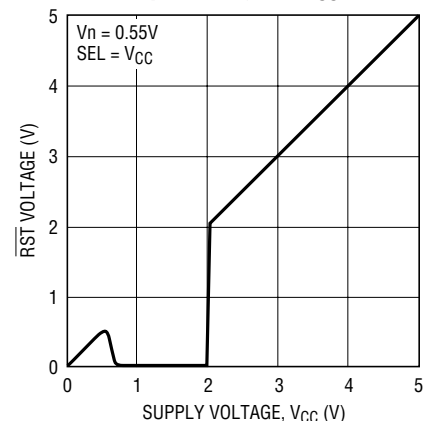
\overline{\text{RST}} Output Voltage vs V_{CC}
