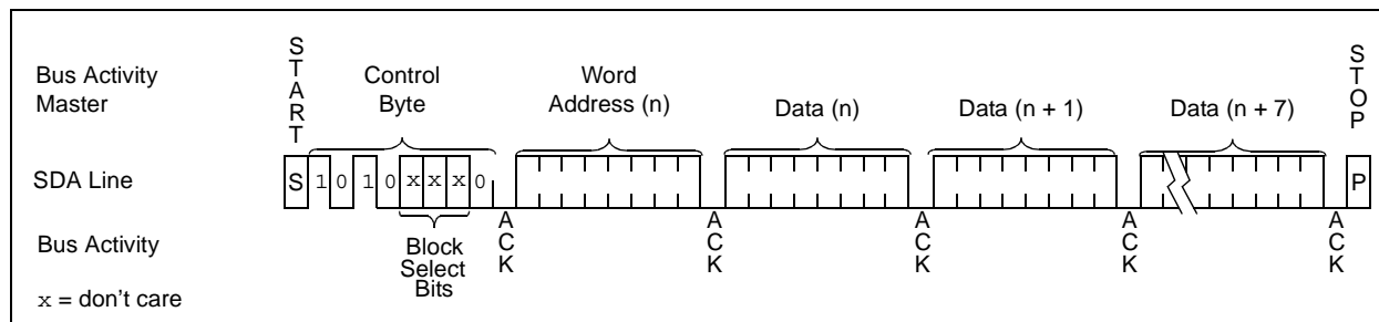
FIGURE 4-2: PAGE WRITE
