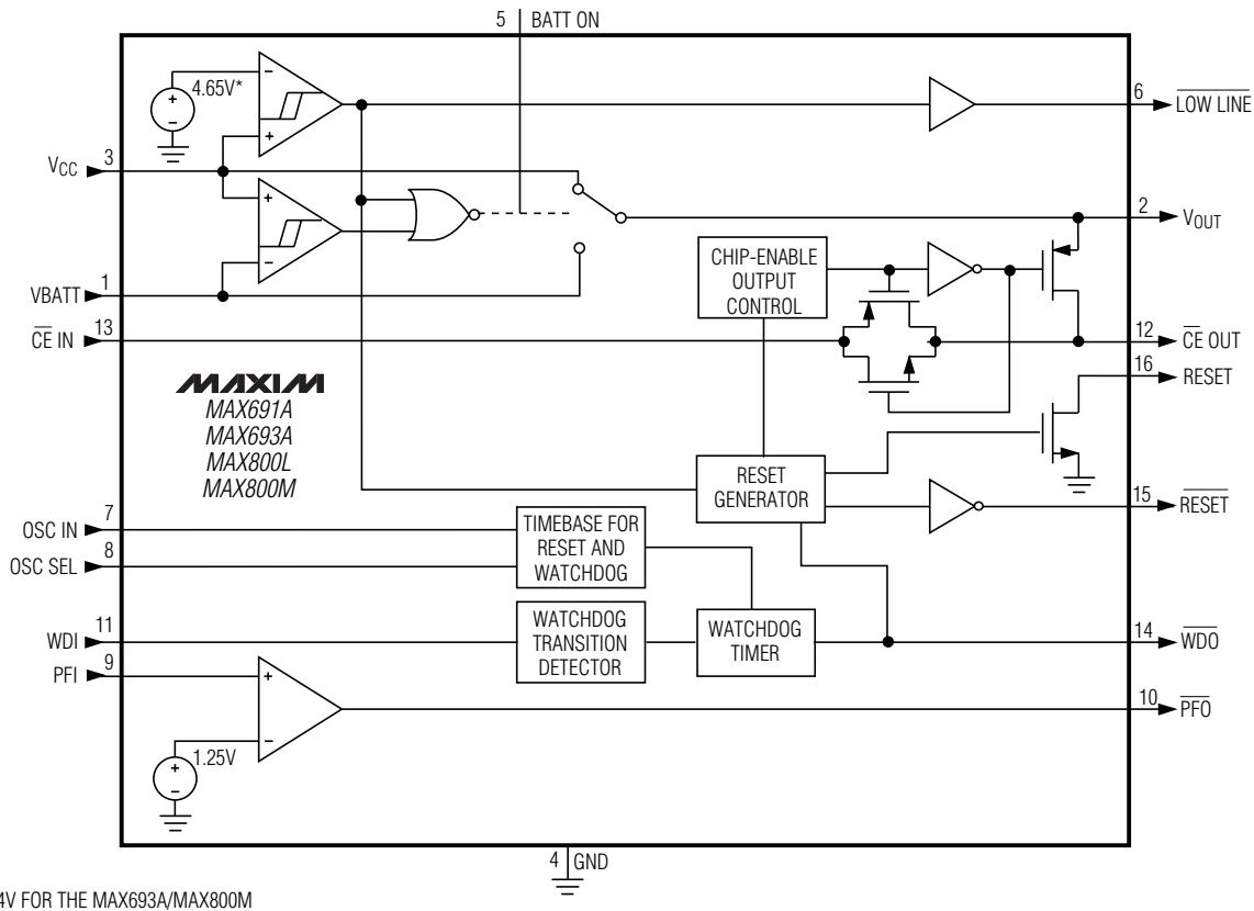
Figure 4. MAX691A/MAX693A/MAX800L/MAX800M Block Diagram
