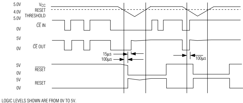
Figure 5. Reset and Chip-Enable Timing
