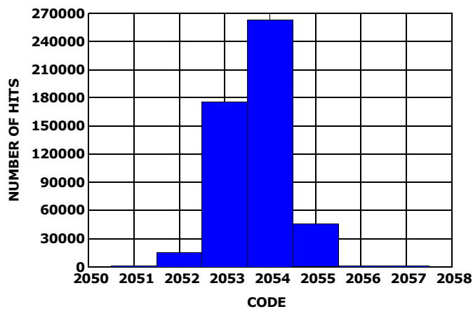
FIGURE 13. NOISE HISTOGRAM
