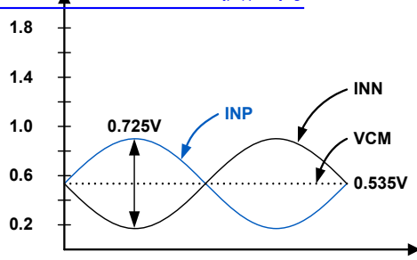
FIGURE 25. ANALOG INPUT RANGE
