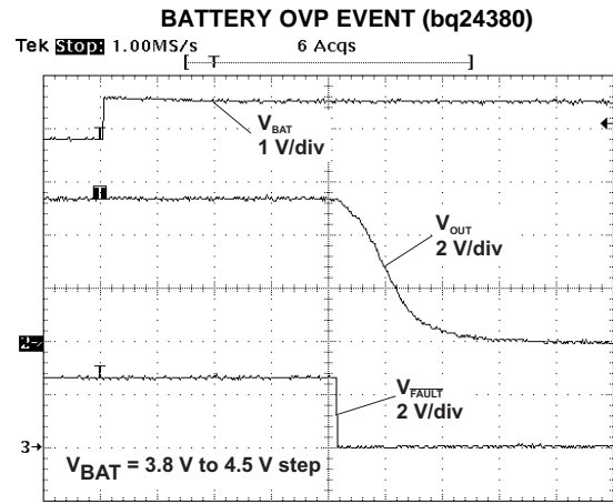
t - Time - 50 \mu s/div Figure 8.
