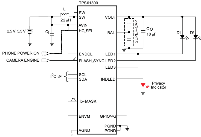
Figure 4. TPS61300, Typical Application
