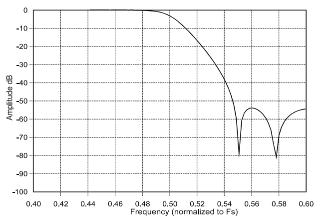
Figure 26. SSM Transition Band
