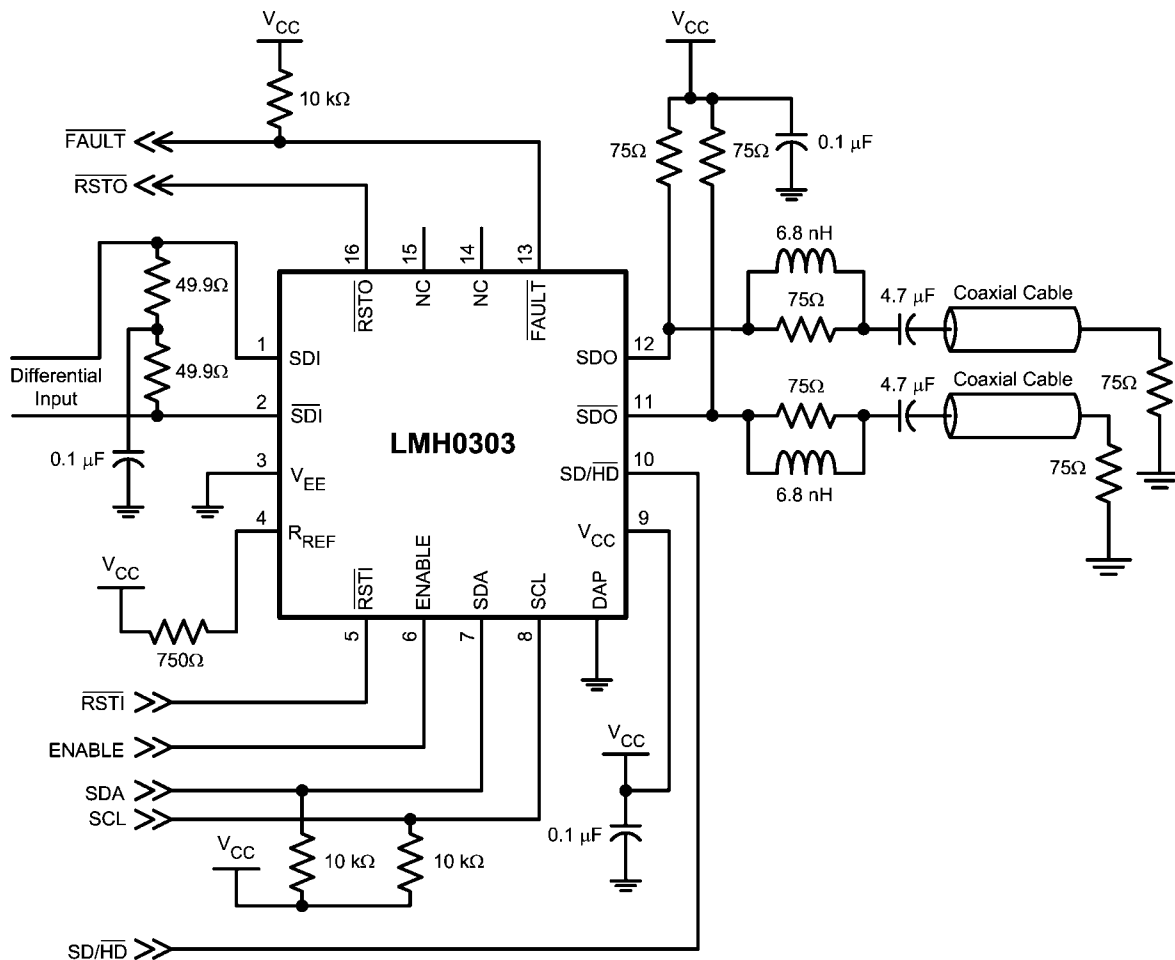
FIGURE 1. Application Circuit
