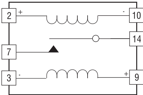
Figure 1. Electrical Configuration
