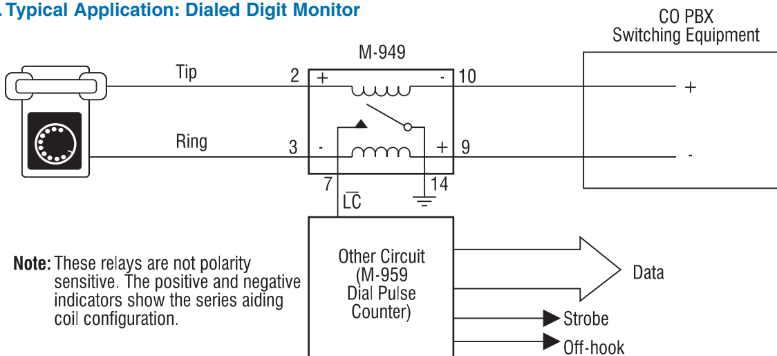
Figure 2. Typical Application: Dialed Digit Monitor
