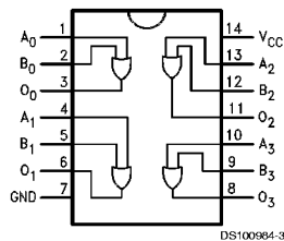
Pin Assignment for DIP and Flatpak
