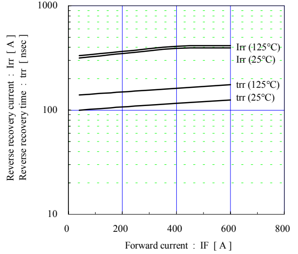
Reverse recovery characteristics (typ.) Vcc=600V, VGE=±15V, Rg=1.5Ω
