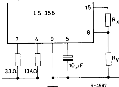
Fig. 14 - Application circuit with fixed gain operation
