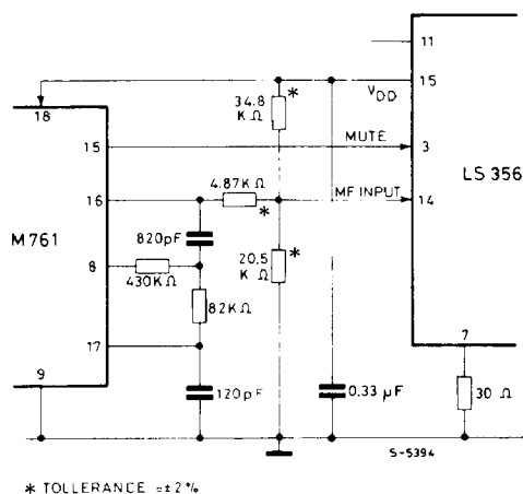
Fig. 10 – Application circuit with multifrequency (EUROPE I)
