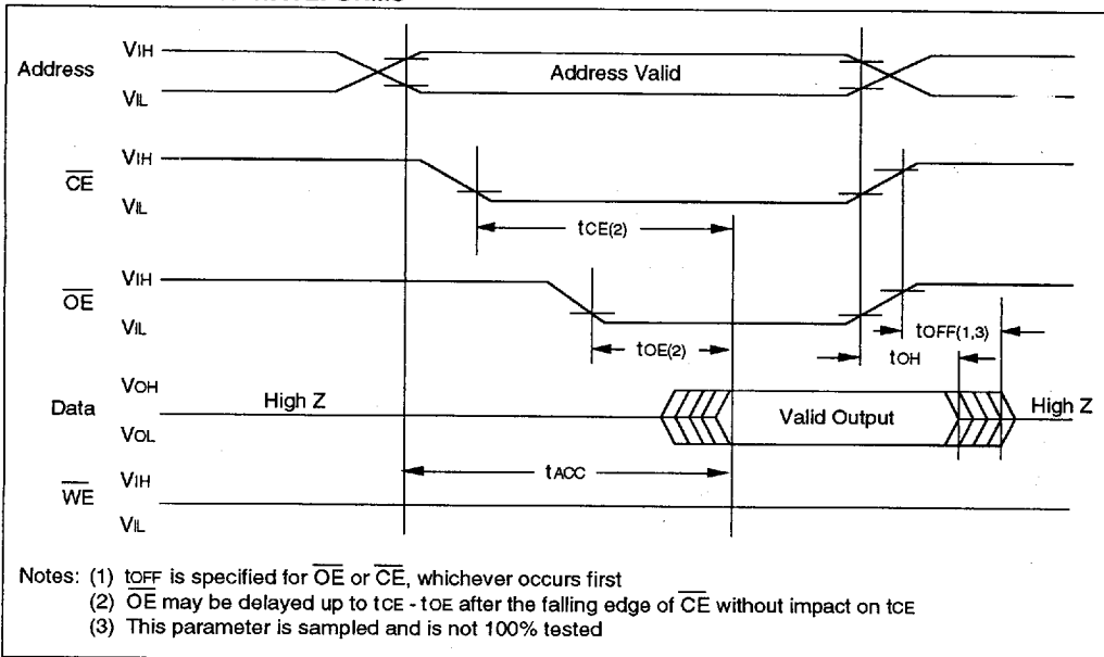
FIGURE 1-1: READ WAVEFORMS
