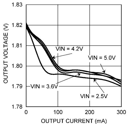
Output Voltage vs. Output Current (V_{OUT} = 1.8V)
