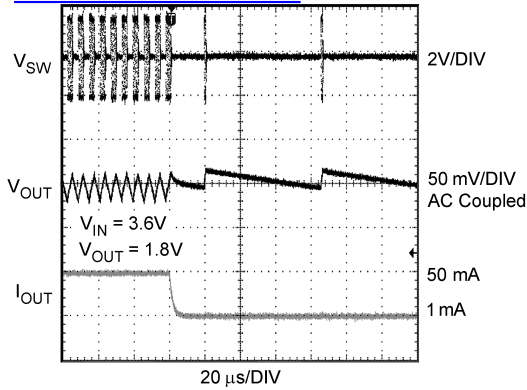
Load Transient Response ( V_{OUT} = 1.8V ) PFM Mode (10mA to 1mA)
