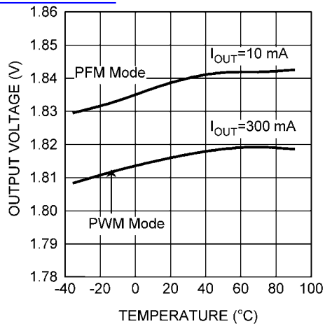
Output Voltage vs. Temperature 查询"LM3679"供应商 ( V_{OUT} = 1.8V )
