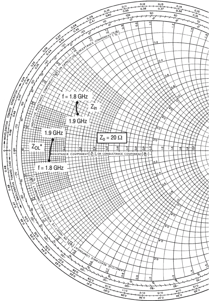
Figure 1. Input and Output Impedances with Circuit Tuned for Maximum Gain @ V CC = 26 V, I CQ = 150 mA, P out = 30 W
